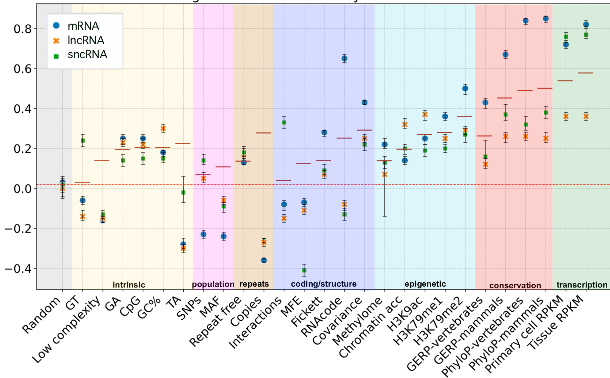
Kolmogorov-Smirnov statistic by feature and dataset
